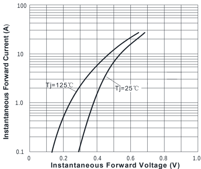
FIG.3: Forward Voltage
