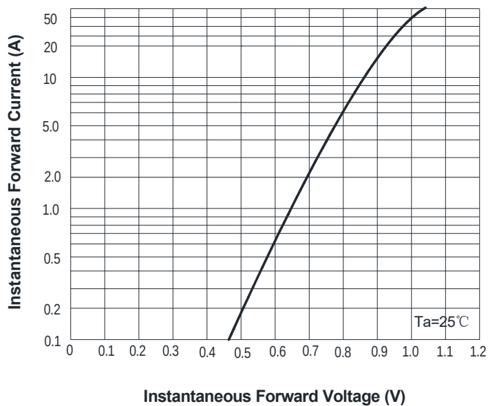
FIG3: Forward Voltage
