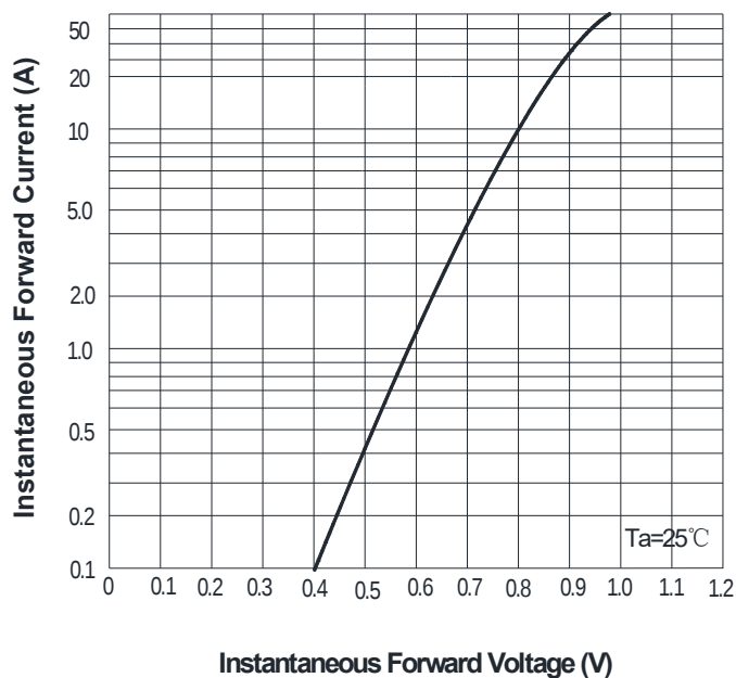
FIG3: Forward Voltage
