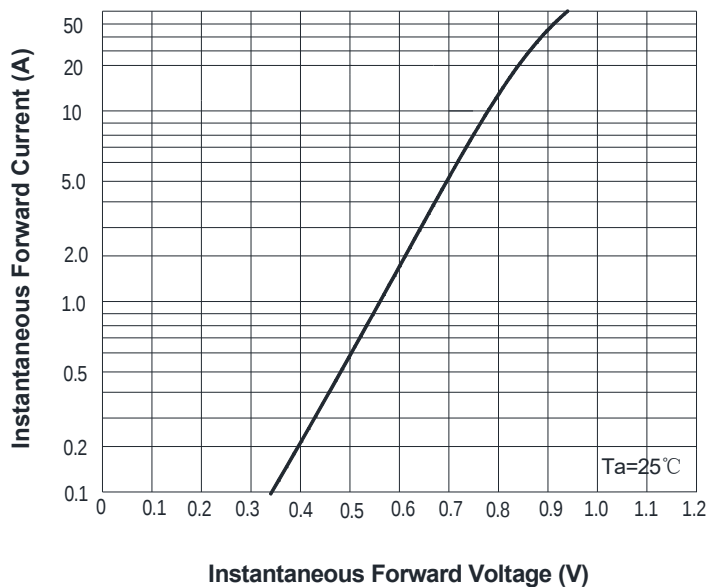
FIG3: Forward Voltage
