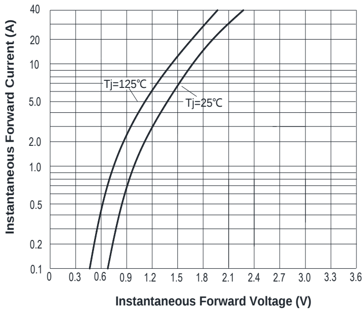
FIG3: Forward Voltage
