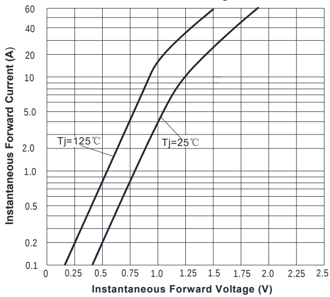
FIG3: Forward Voltage
