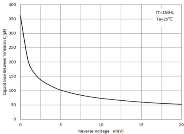
Fig 3: Capacitance Capability
