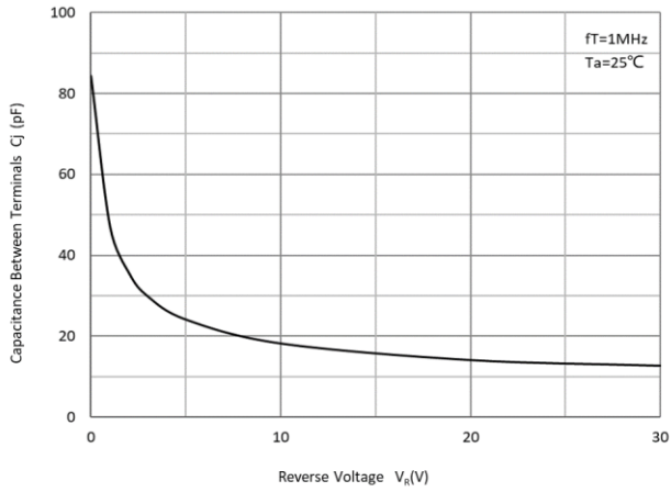
Fig 3: Capacitance Capability
