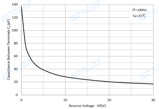
Fig 3: Capacitance Capability
