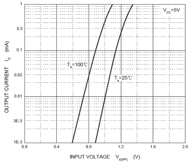
OFF Characteristics
