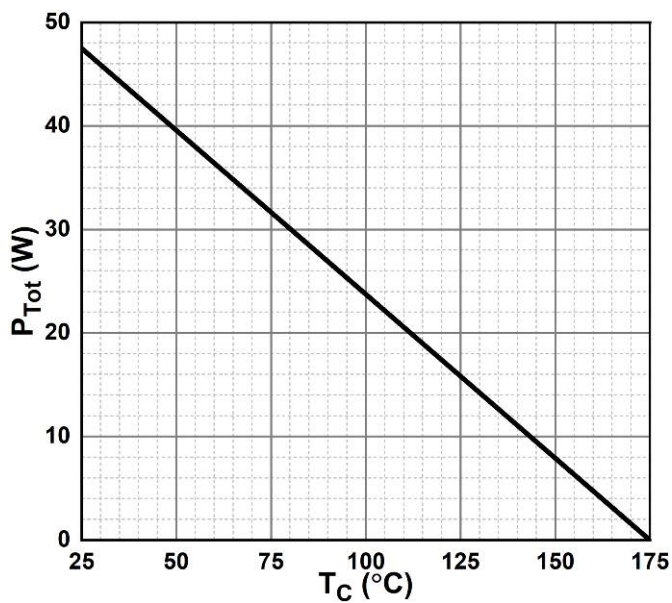
Figure 6. Power Derating
