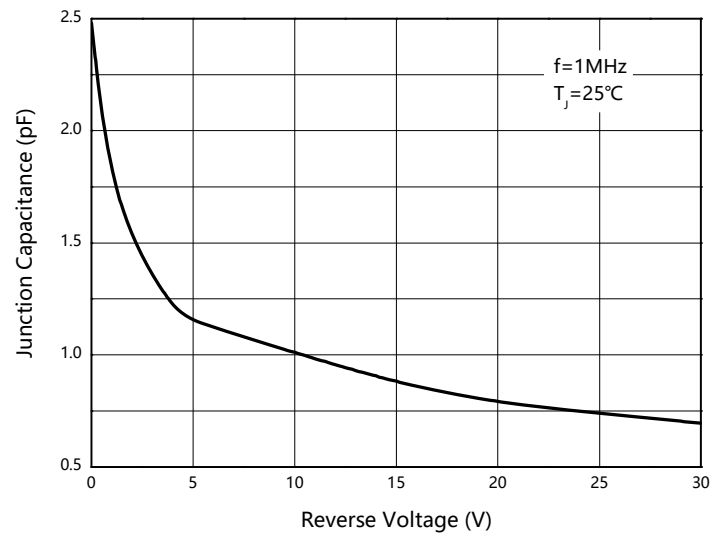
Fig.2: Capacitance Characteristics
