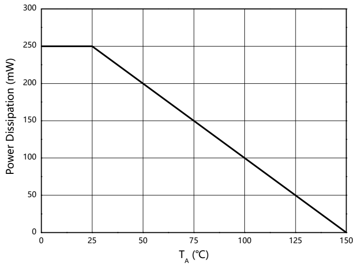
Fig.1: P_D - T_A
