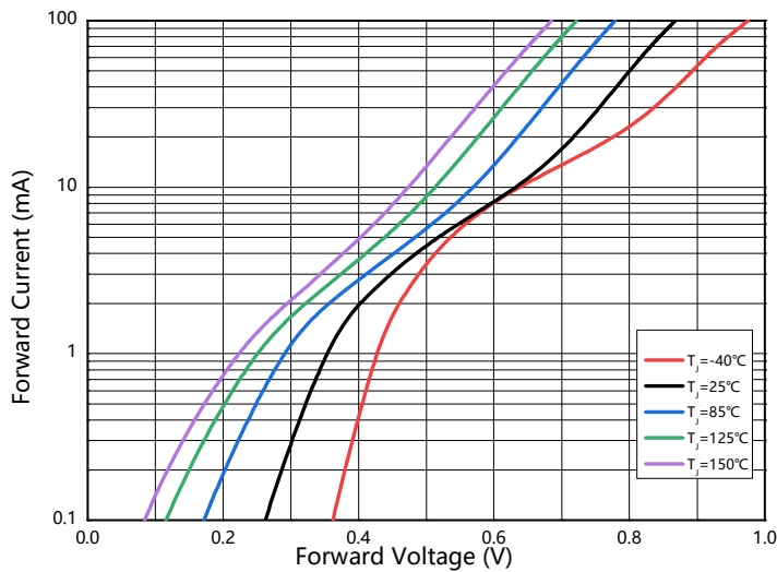
Fig.3: Forward Characteristics
