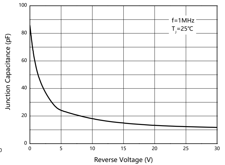
Fig.2: Capacitance Characteristics
