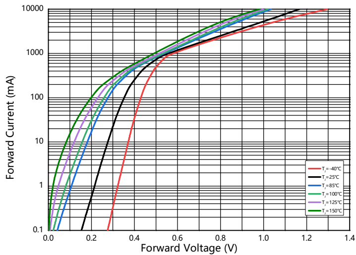
Fig.3: Forward Characteristics
