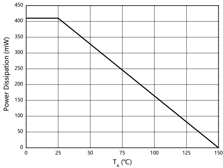
Fig.1: P_D - T_A
