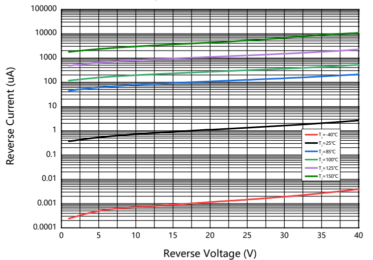
Fig.4: Reverse Characteristic
