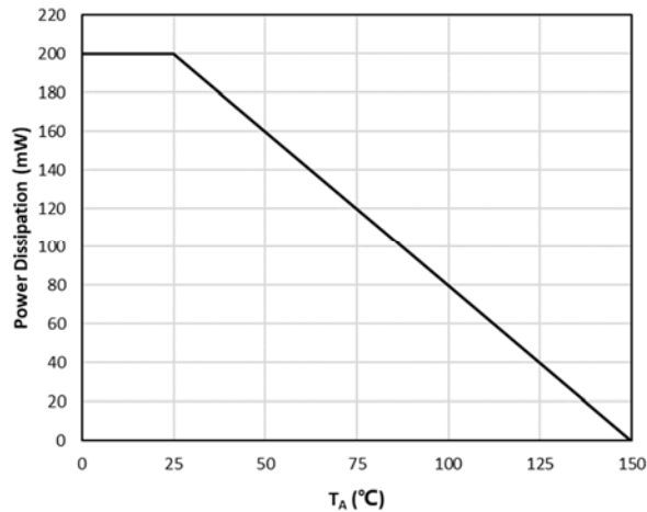
Fig.1: P_D-T_A
