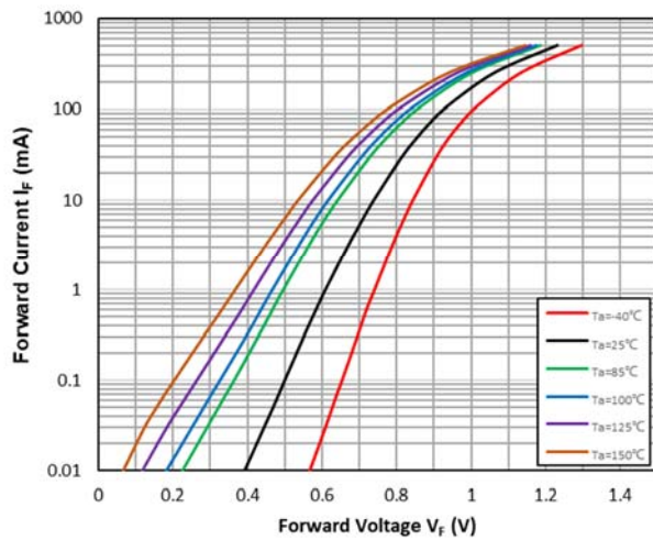
Fig.3: Forward Characteristic
