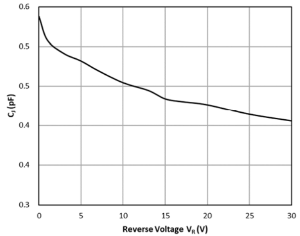
Fig.2: Capacitance Characteristic
