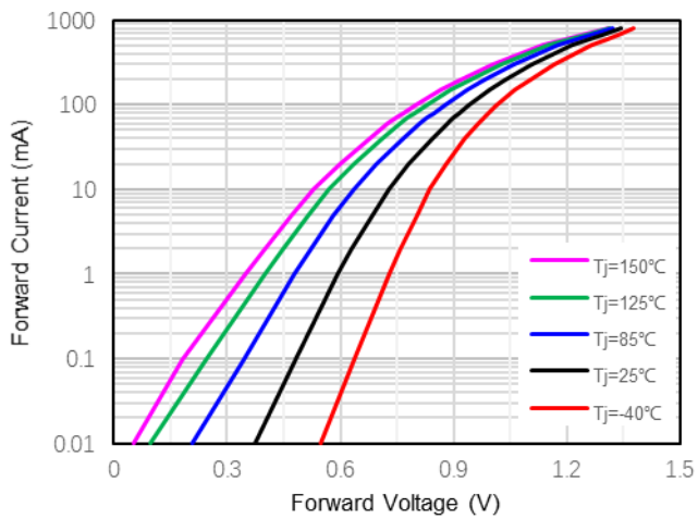
Fig.3: Forward Characteristics
