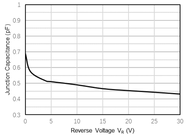
Fig.2: Capacitance Characteristics
