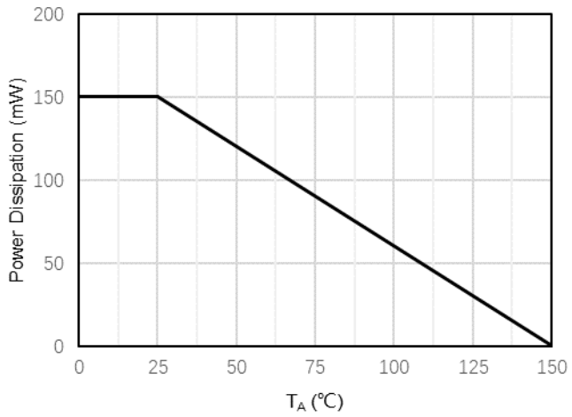
Fig.1: P_D - T_A
