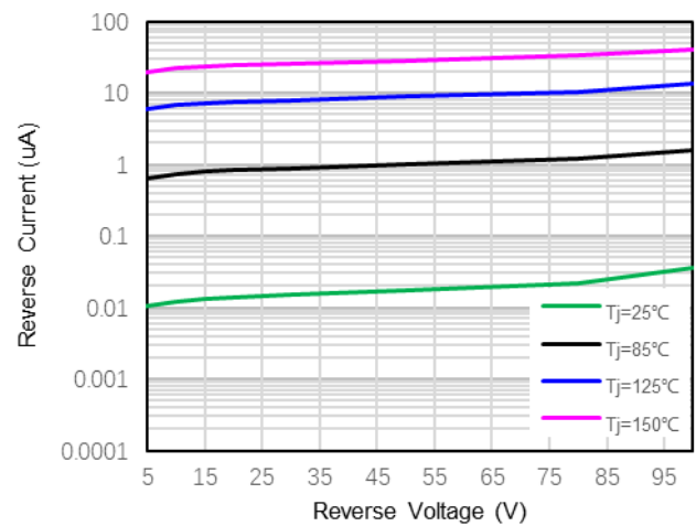
Fig.4: Reverse Characteristics
