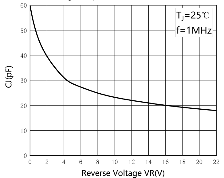
Fig.6: Capacitance Characteristics
