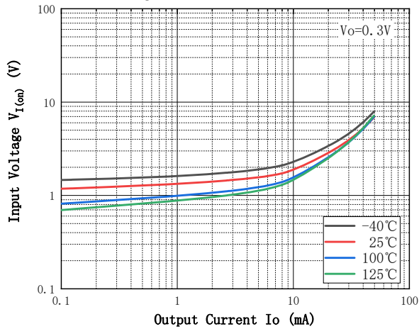
Fig.1 - ON Characteristics
