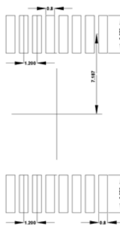
SUGGESTED SOLDER PAD LAYOUT
