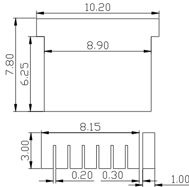
SUGGESTED SOLDER PAD LAYOUT
