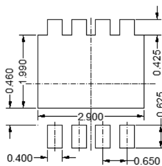
Suggested Solder Pad Layout Top View
