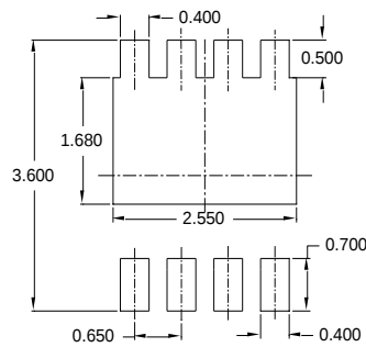
SUGGESTED SOLDER PAD LAYOUT
