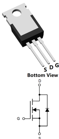
TO-220
