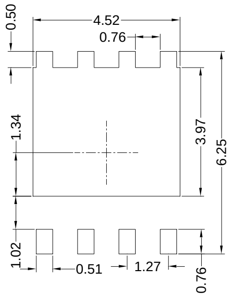
Suggested Solder Pad Layout Top View
