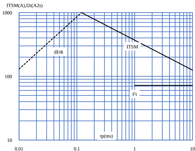
FIG.5: Non-repetitive surge peak on-state current for a sinusoidal pulse with width tp<20ms , and corresponding value of I^2t ( I - II - III: dI/dt < 50A/\mu s ;
