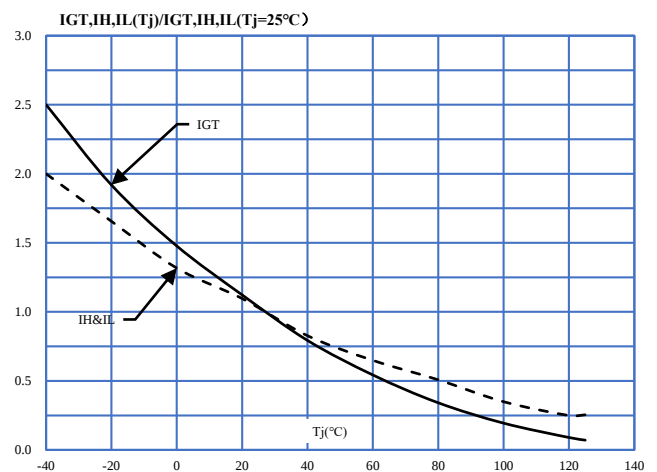
FIG.6: Relative variations of gate trigger current, holding current and latching current
