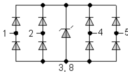
DFN2510-10L
