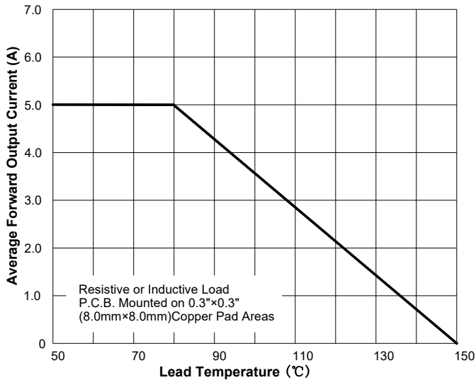
FIG.1: Io-TL Curve
