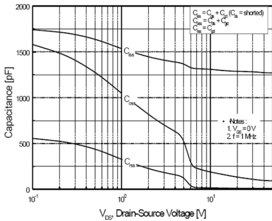
Fig. 5 Capacitance Characteristics
